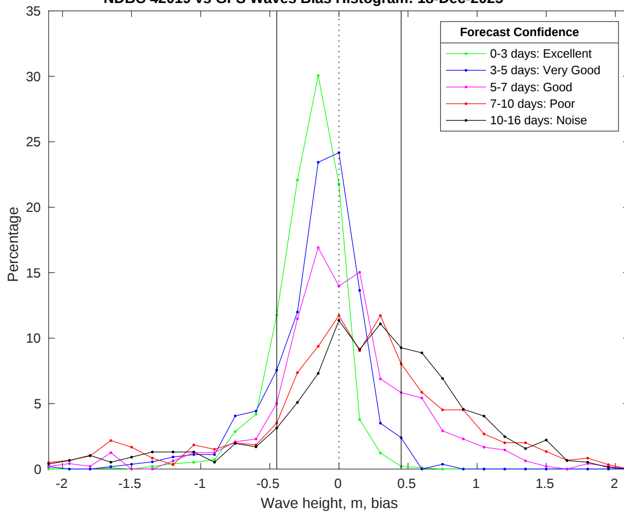
NDBC 42019 vs GFS Waves Bias Histogram: 18-Dec-2025
