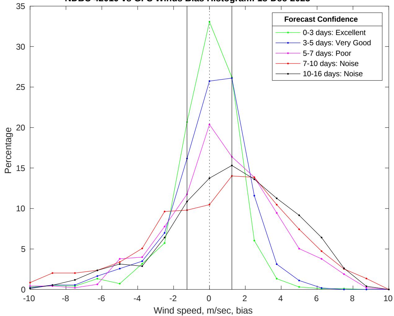
NDBC 42019 vs GFS Winds Bias Histogram: 18-Dec-2025
