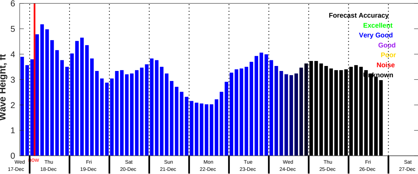
CMEMS Wave Forecast for NDBC 42019 from 17-Dec-2025 18:00:00 to 27-Dec-2025 18:00:00
