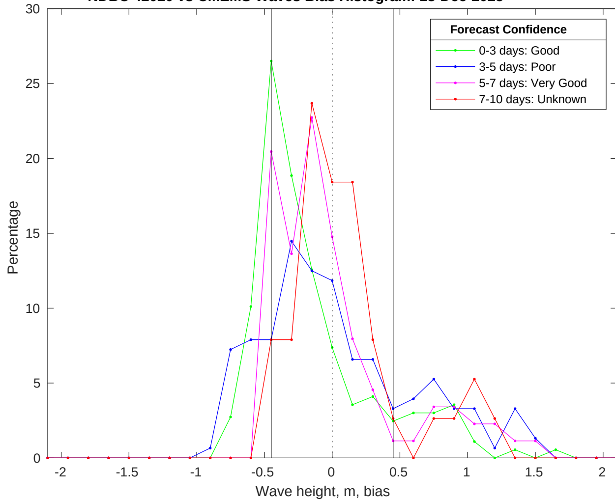
NDBC 42020 vs CMEMS Waves Bias Histogram: 18-Dec-2025
