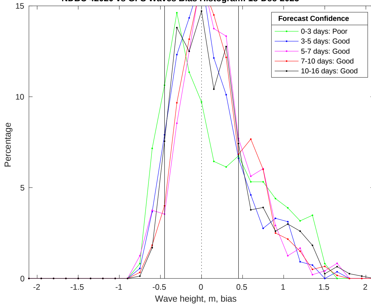
NDBC 42020 vs GFS Waves Bias Histogram: 18-Dec-2025
