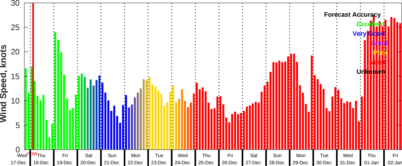
GFS Wind Speed Forecast for NDBC 42020 from 17-Dec-2025 18:00:00 to 02-Jan-2026 18:00:00
