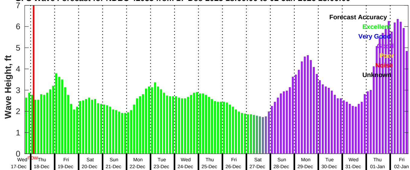
GFS Wave Forecast for NDBC 42035 from 17-Dec-2025 18:00:00 to 02-Jan-2026 18:00:00
