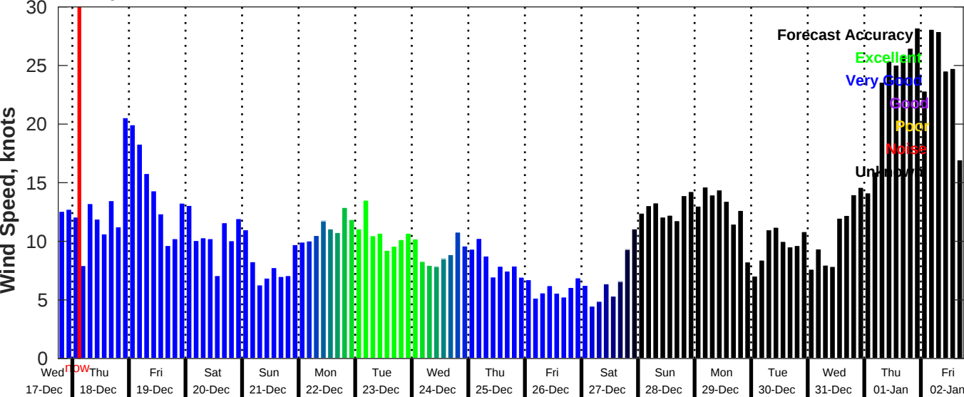
GFS Wind Speed Forecast for NDBC 42035 from 17-Dec-2025 18:00:00 to 02-Jan-2026 18:00:00
