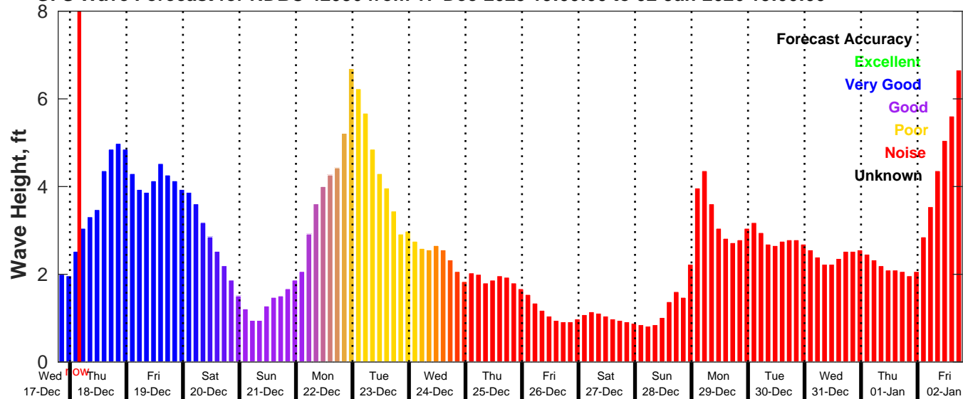
GFS Wave Forecast for NDBC 42036 from 17-Dec-2025 19:00:00 to 02-Jan-2026 19:00:00
