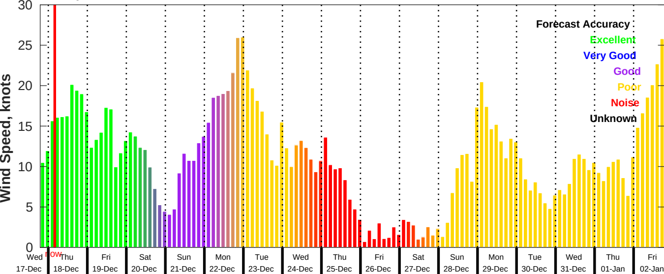
GFS Wind Speed Forecast for NDBC 42036 from 17-Dec-2025 19:00:00 to 02-Jan-2026 19:00:00
