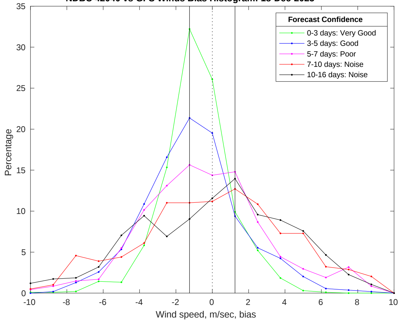
NDBC 42040 vs GFS Winds Bias Histogram: 18-Dec-2025
