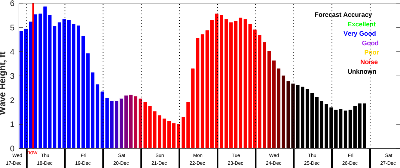
CMEMS Wave Forecast for NDBC 42040 from 17-Dec-2025 19:00:00 to 27-Dec-2025 19:00:00
