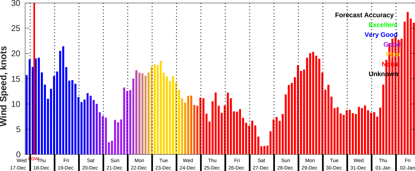
GFS Wind Speed Forecast for NDBC 42040 from 17-Dec-2025 19:00:00 to 02-Jan-2026 19:00:00
