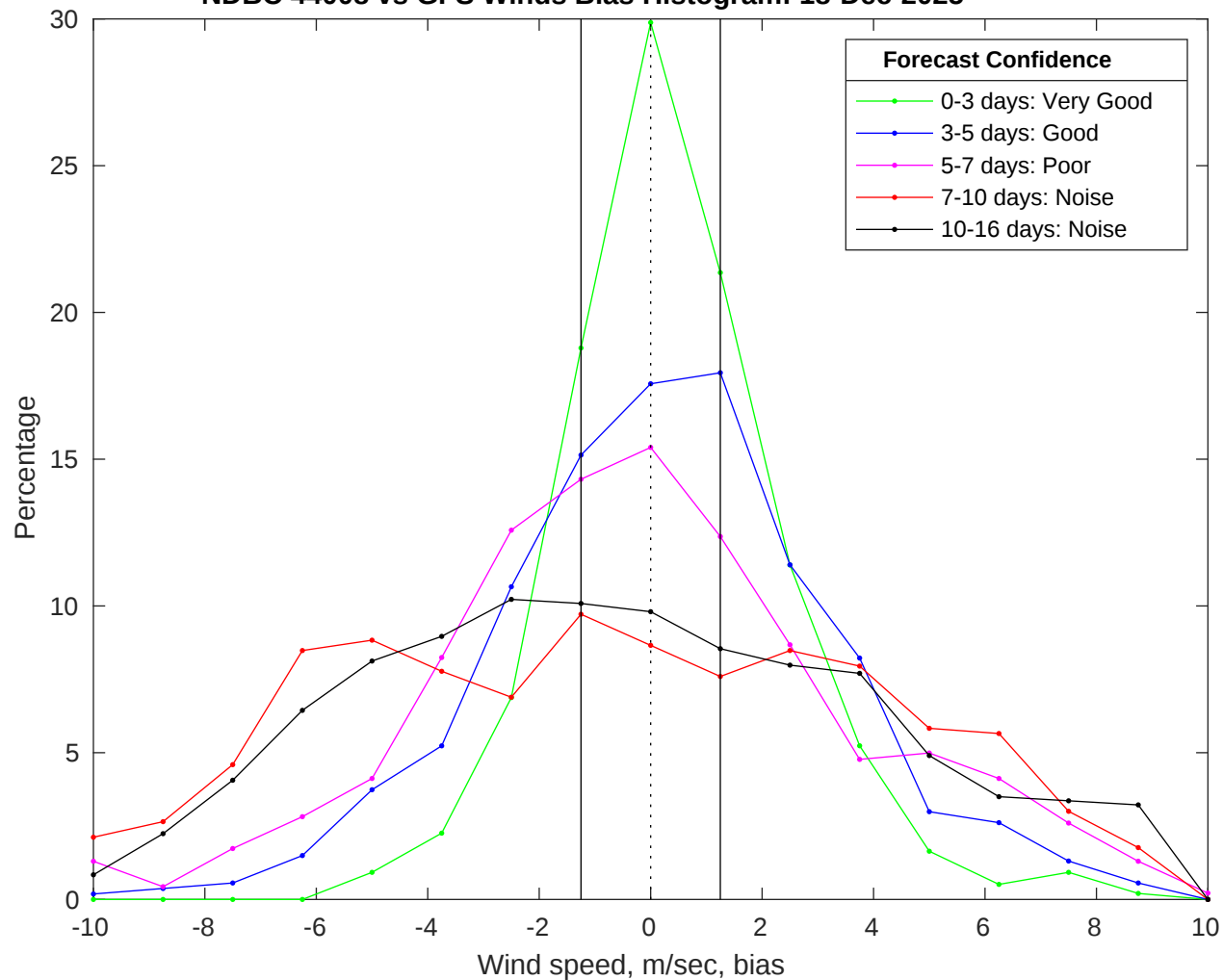
NDBC 44008 vs GFS Winds Bias Histogram: 18-Dec-2025
