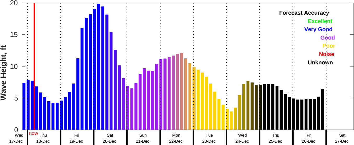
CMEMS Wave Forecast for NDBC 44008 from 17-Dec-2025 20:00:00 to 27-Dec-2025 20:00:00
