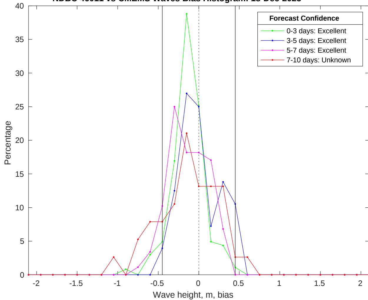
NDBC 46011 vs CMEMS Waves Bias Histogram: 18-Dec-2025
