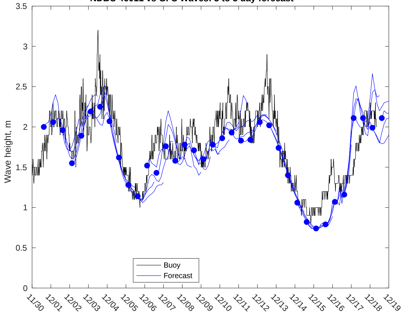
NDBC 46011 vs GFS Waves: 3 to 5 day forecast
