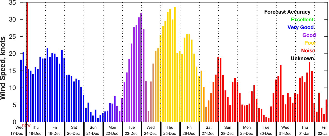
GFS Wind Speed Forecast for NDBC 46011 from 17-Dec-2025 16:00:00 to 02-Jan-2026 16:00:00
