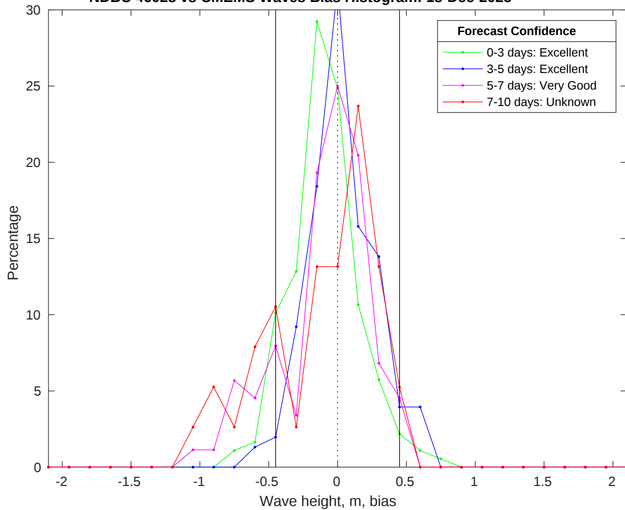
NDBC 46028 vs CMEMS Waves Bias Histogram: 18-Dec-2025
