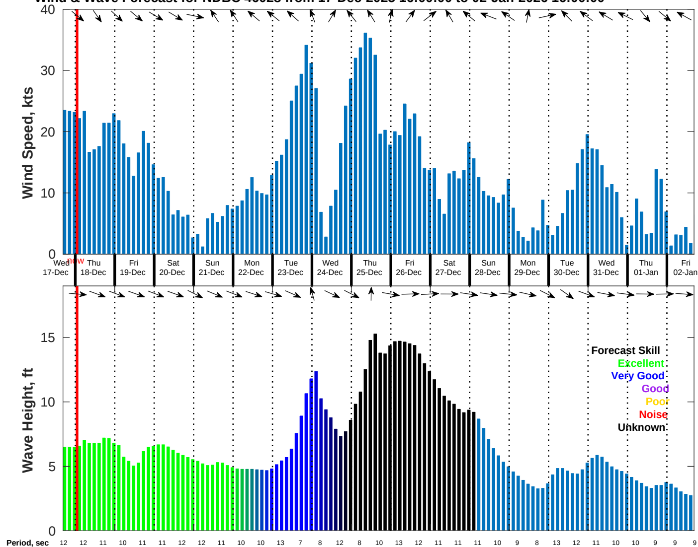
Wind & Wave Forecast for NDBC 46028 from 17-Dec-2025 16:00:00 to 02-Jan-2026 16:00:00
