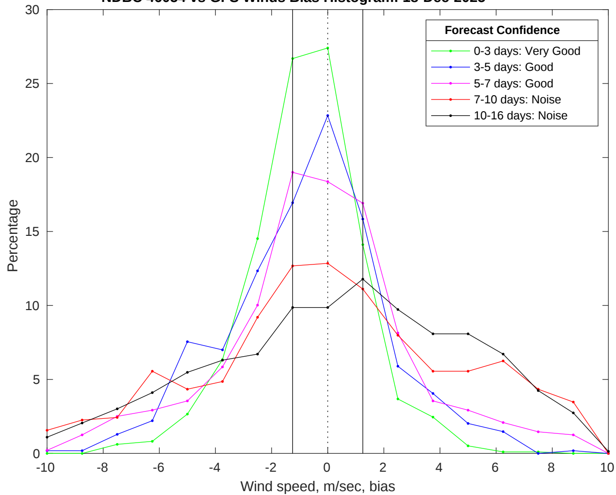
NDBC 46054 vs GFS Winds Bias Histogram: 18-Dec-2025
