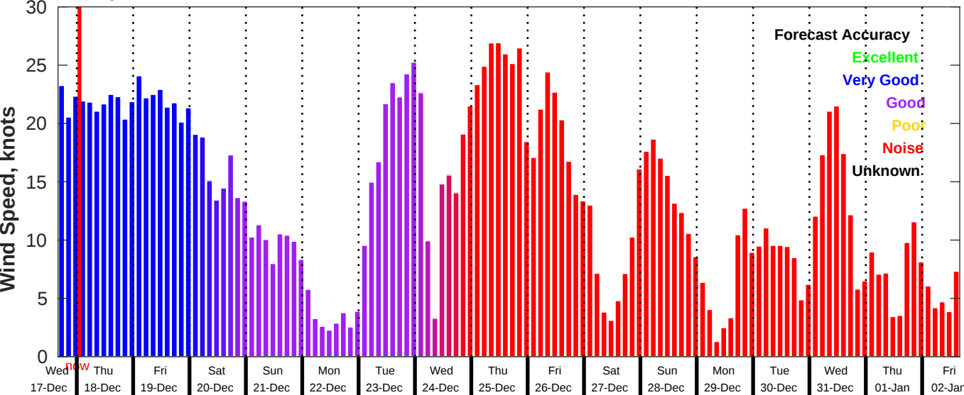
GFS Wind Speed Forecast for NDBC 46054 from 17-Dec-2025 16:00:00 to 02-Jan-2026 16:00:00
