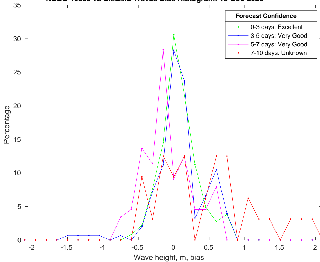
NDBC 46059 vs CMEMS Waves Bias Histogram: 18-Dec-2025
