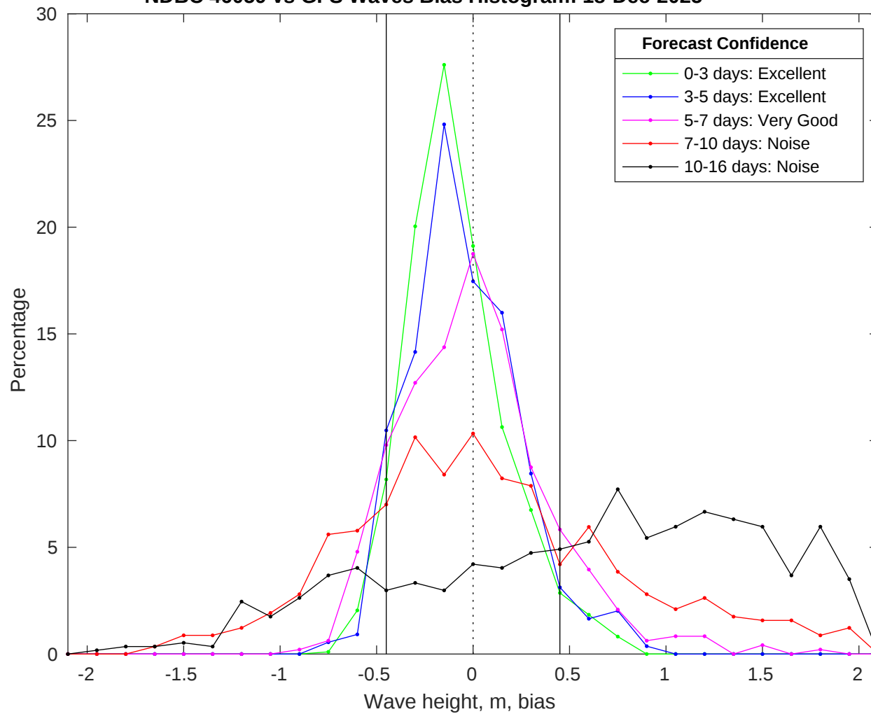
NDBC 46059 vs GFS Waves Bias Histogram: 18-Dec-2025
