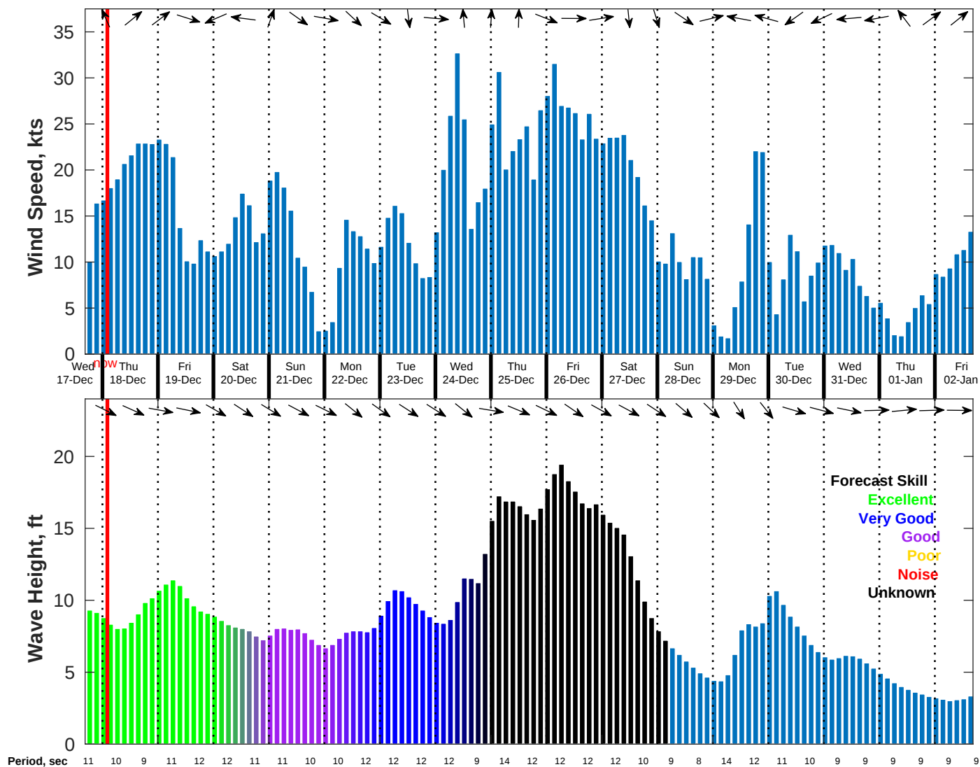
Wind & Wave Forecast for NDBC 46059 from 17-Dec-2025 17:00:00 to 02-Jan-2026 17:00:00
