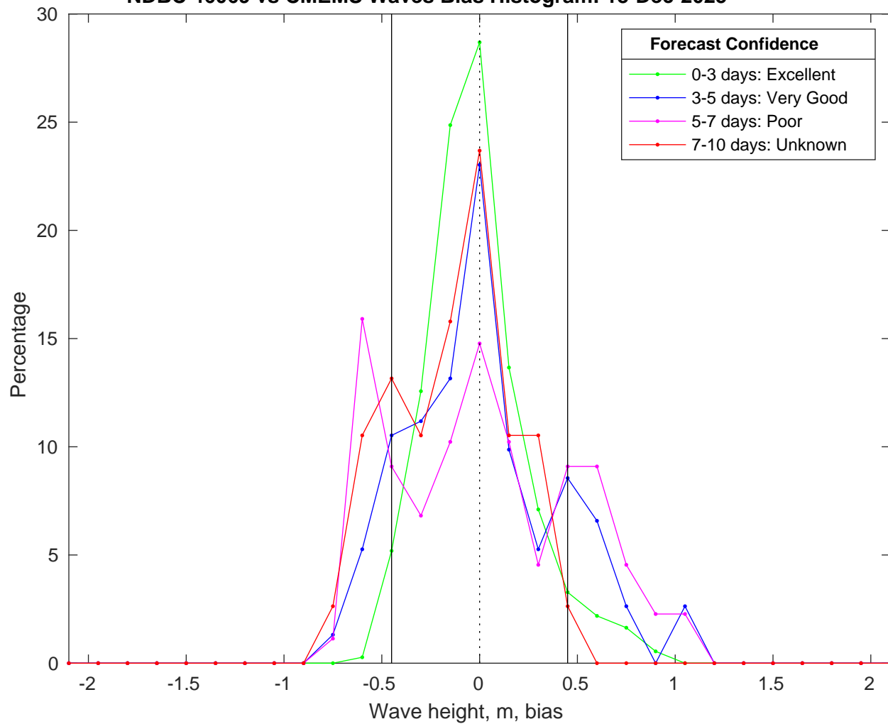
NDBC 46069 vs CMEMS Waves Bias Histogram: 18-Dec-2025
