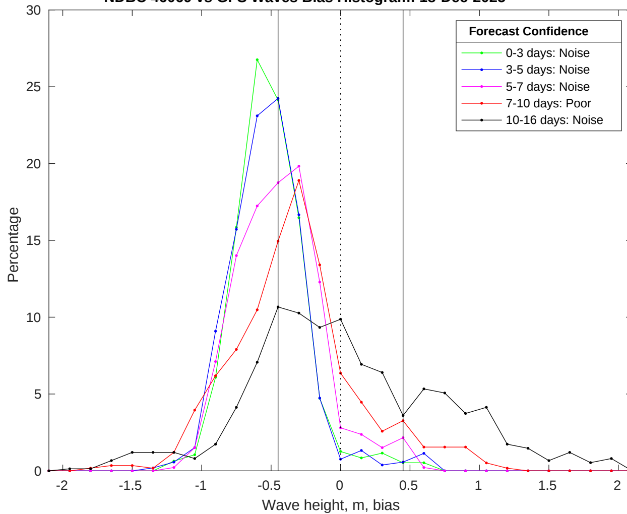
NDBC 46069 vs GFS Waves Bias Histogram: 18-Dec-2025
