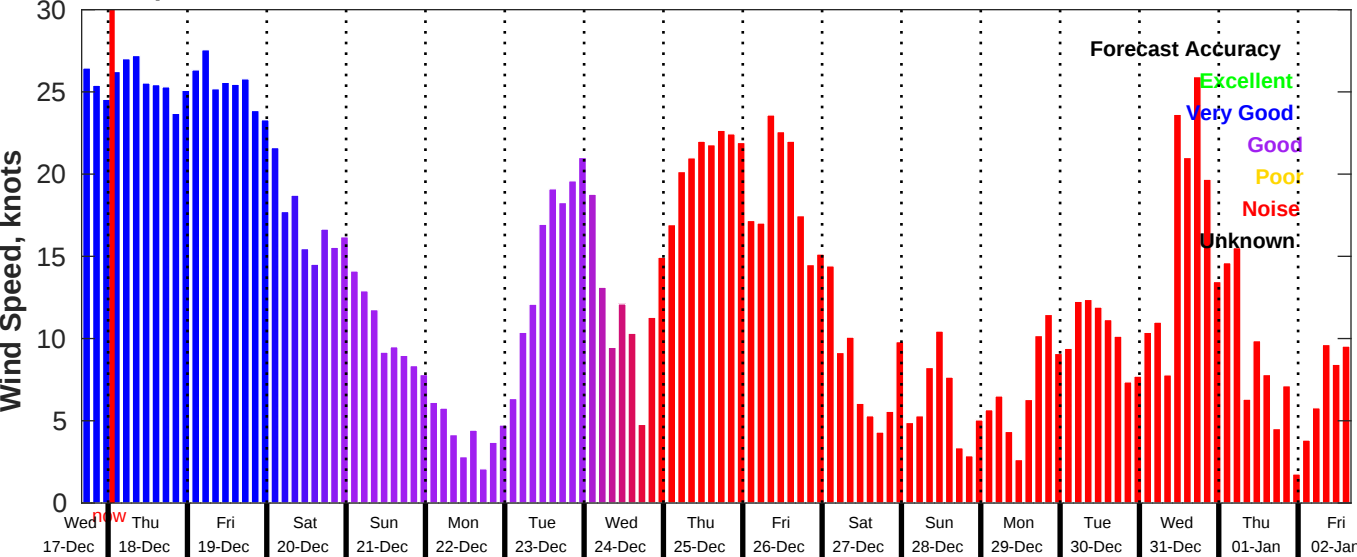
GFS Wind Speed Forecast for NDBC 46069 from 17-Dec-2025 16:00:00 to 02-Jan-2026 16:00:00
