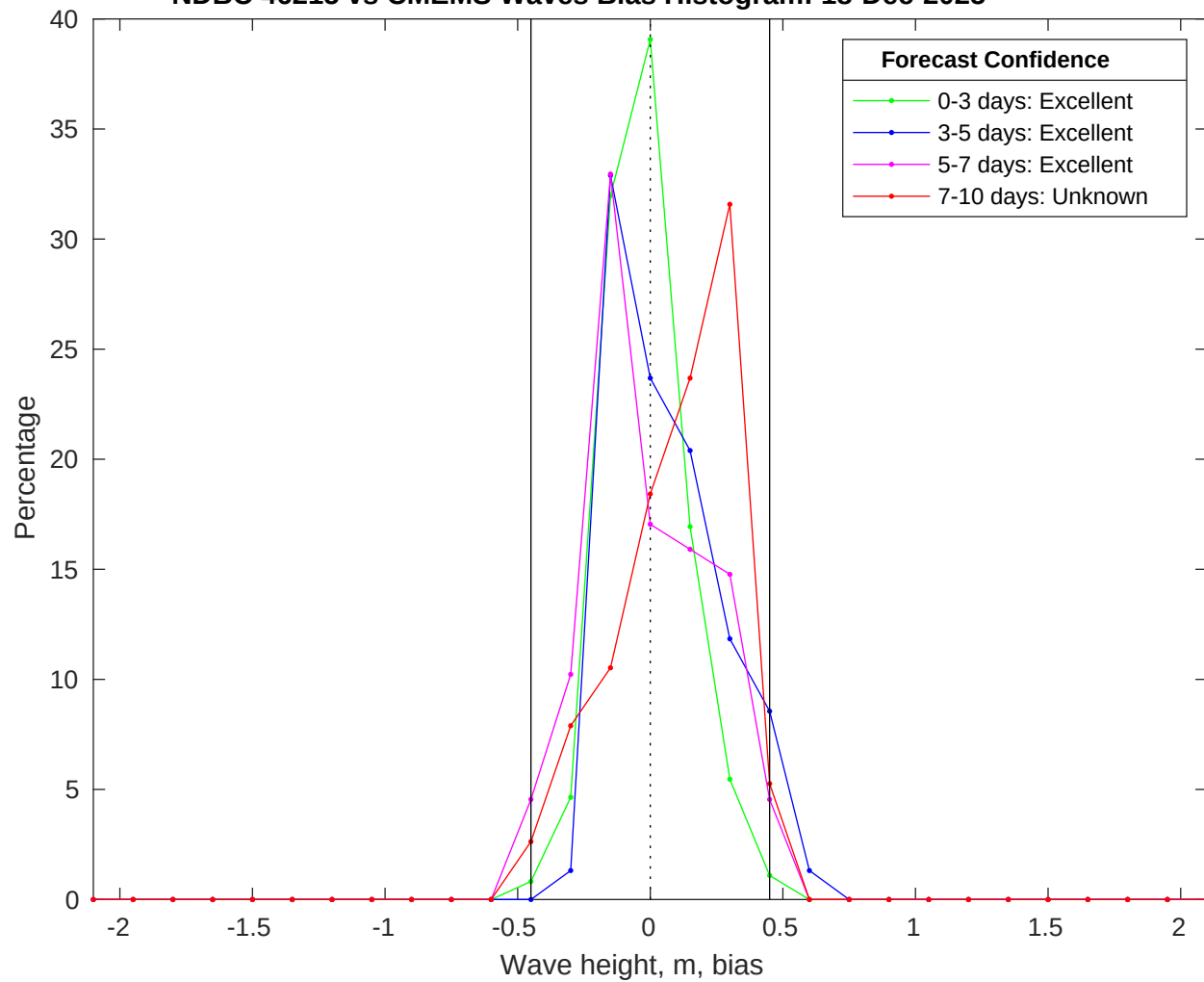
NDBC 46215 vs CMEMS Waves Bias Histogram: 18-Dec-2025
