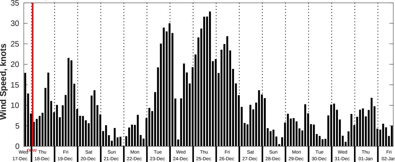
GFS Wind Speed Forecast for NDBC 46215 from 17-Dec-2025 16:00:00 to 02-Jan-2026 16:00:00
