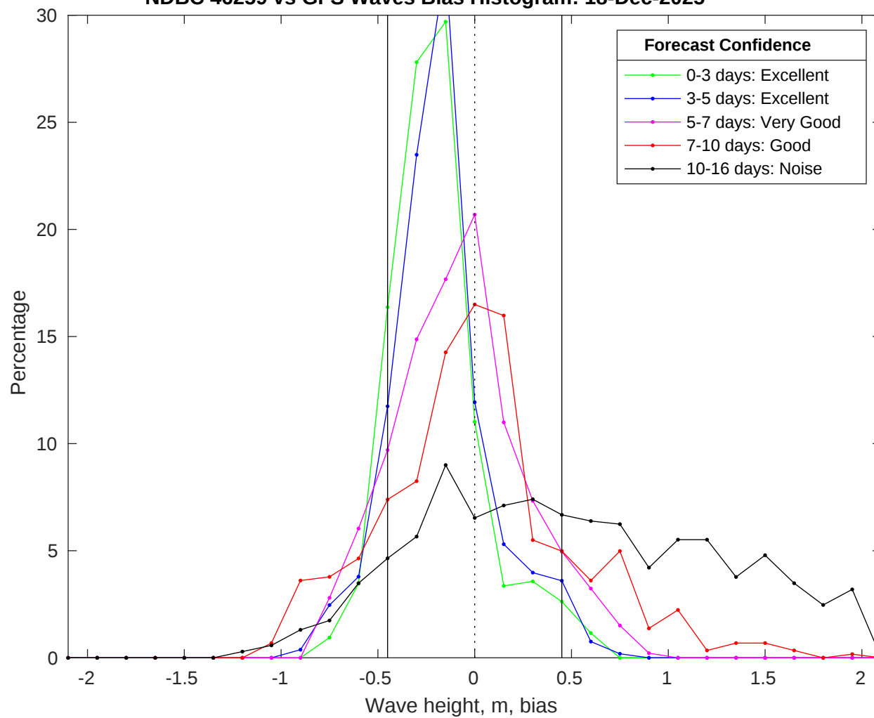
NDBC 46259 vs GFS Waves Bias Histogram: 18-Dec-2025
