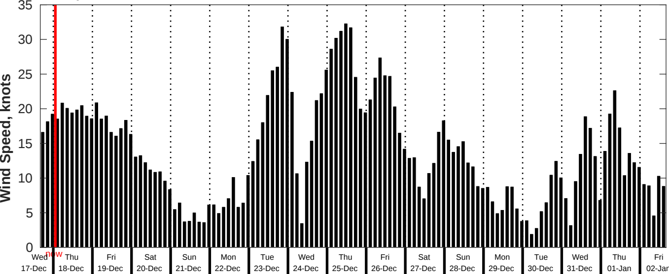
GFS Wind Speed Forecast for NDBC 46259 from 17-Dec-2025 16:00:00 to 02-Jan-2026 16:00:00
