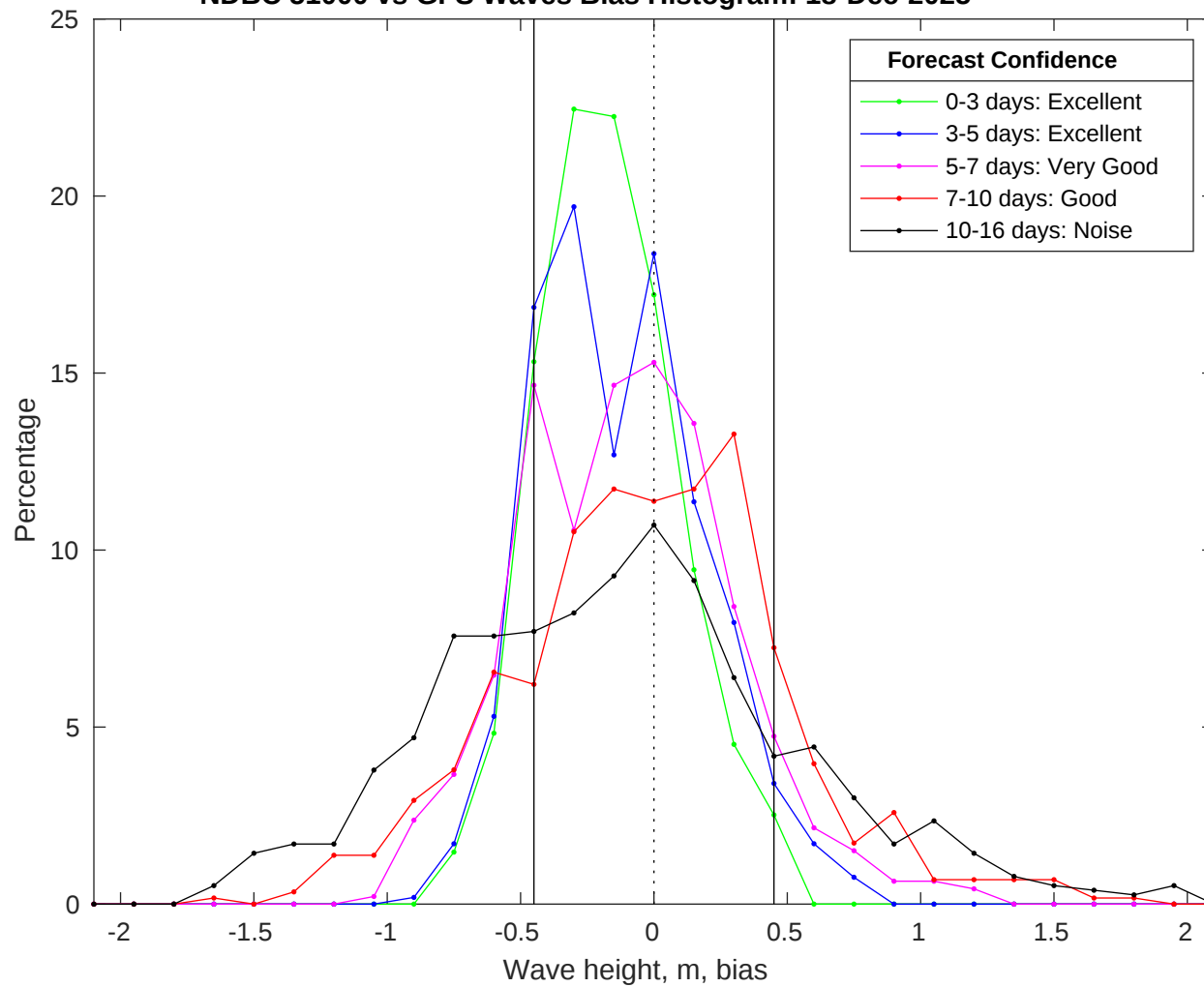
NDBC 51000 vs GFS Waves Bias Histogram: 18-Dec-2025
