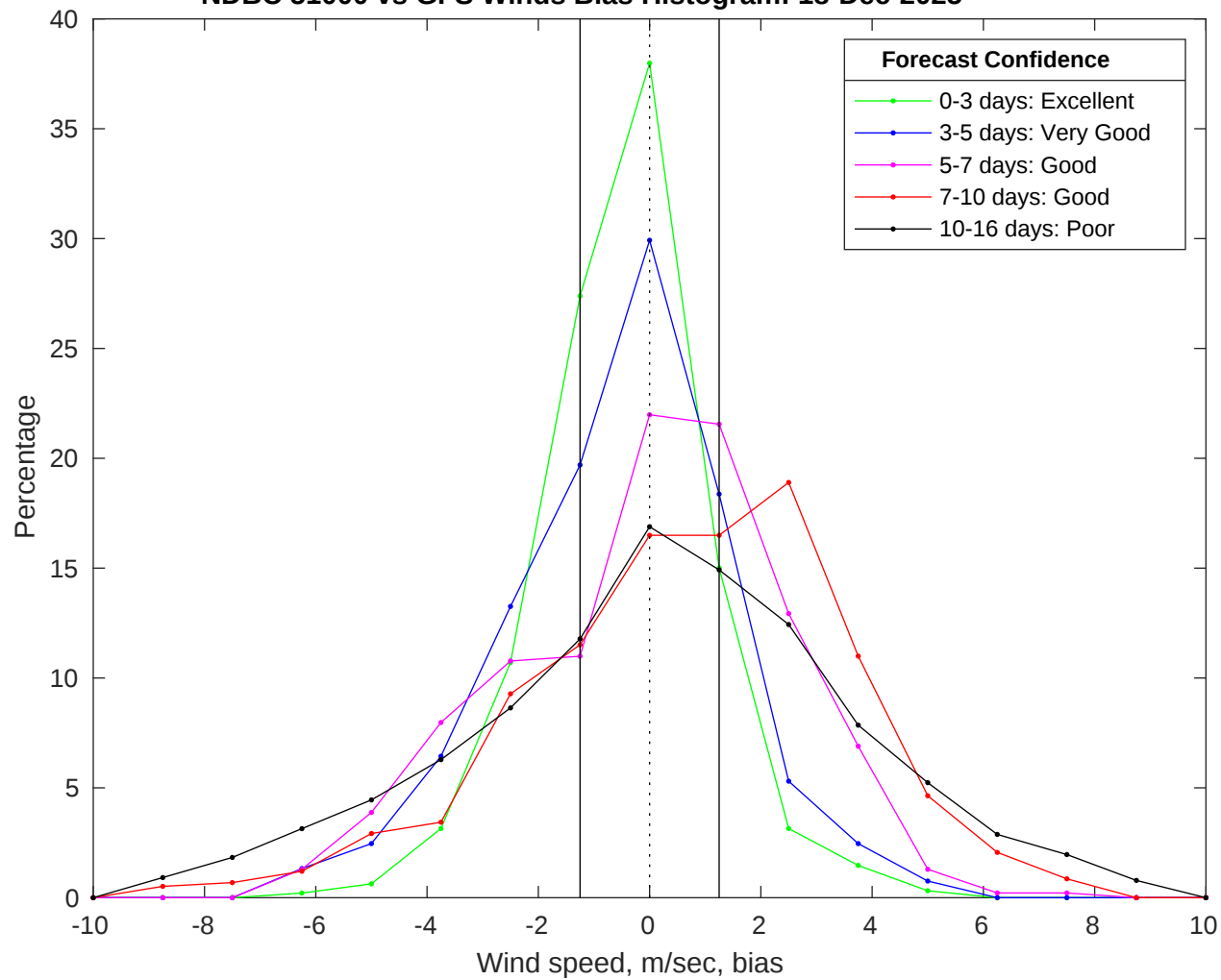
NDBC 51000 vs GFS Winds Bias Histogram: 18-Dec-2025
