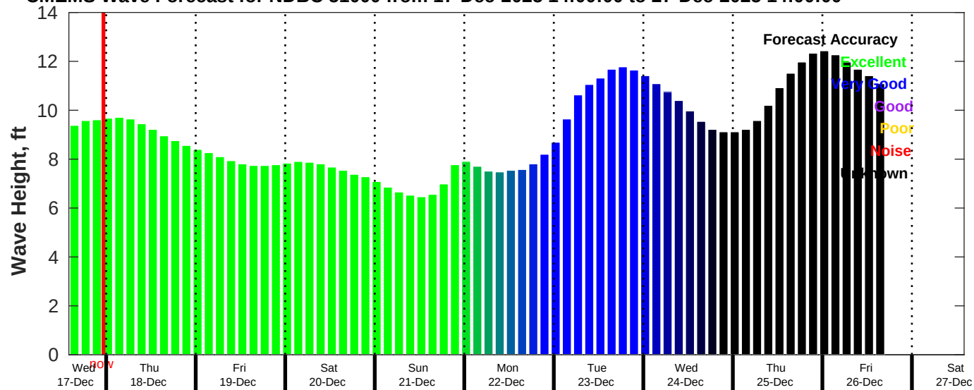
CMEMS Wave Forecast for NDBC 51000 from 17-Dec-2025 14:00:00 to 27-Dec-2025 14:00:00
