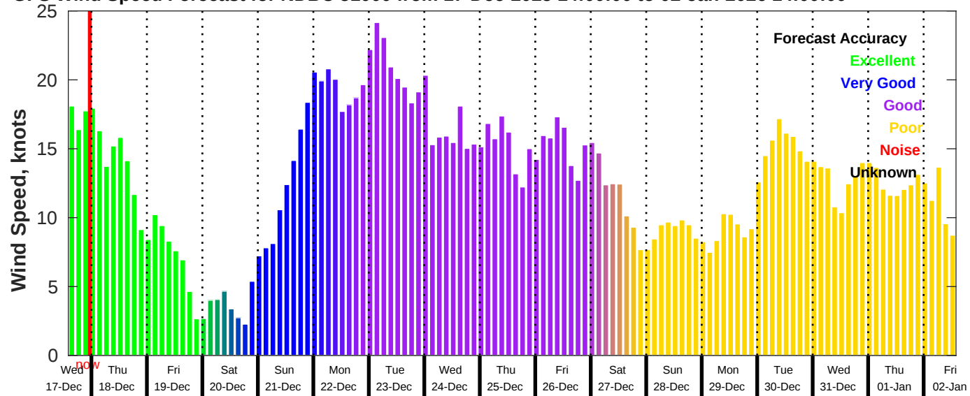
GFS Wind Speed Forecast for NDBC 51000 from 17-Dec-2025 14:00:00 to 02-Jan-2026 14:00:00
