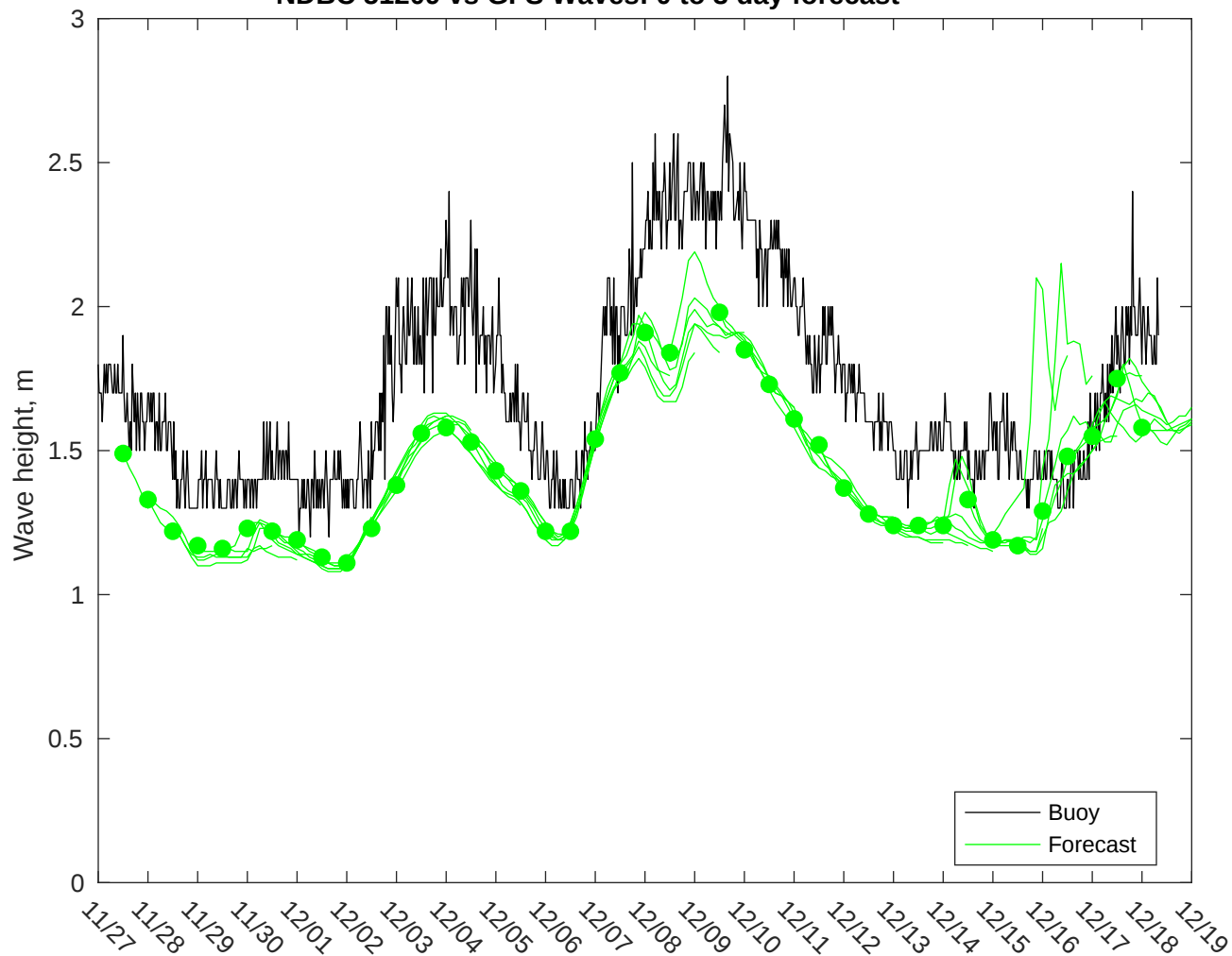
NDBC 51209 vs GFS Waves: 0 to 3 day forecast
