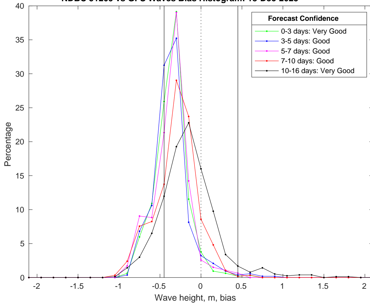
NDBC 51209 vs GFS Waves Bias Histogram: 18-Dec-2025
