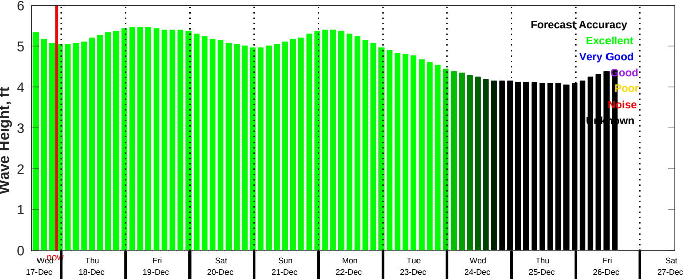
CMEMS Wave Forecast for NDBC 51209 from 17-Dec-2025 13:00:00 to 27-Dec-2025 13:00:00
