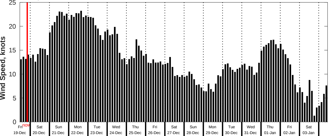
GFS Wind Speed Forecast for NDBC 52211 from 18-Dec-2025 11:00:00 to 03-Jan-2026 11:00:00
