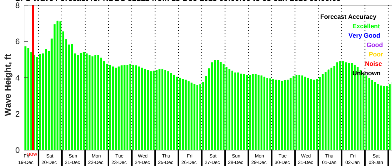
GFS Wave Forecast for NDBC 52212 from 18-Dec-2025 09:00:00 to 03-Jan-2026 09:00:00
