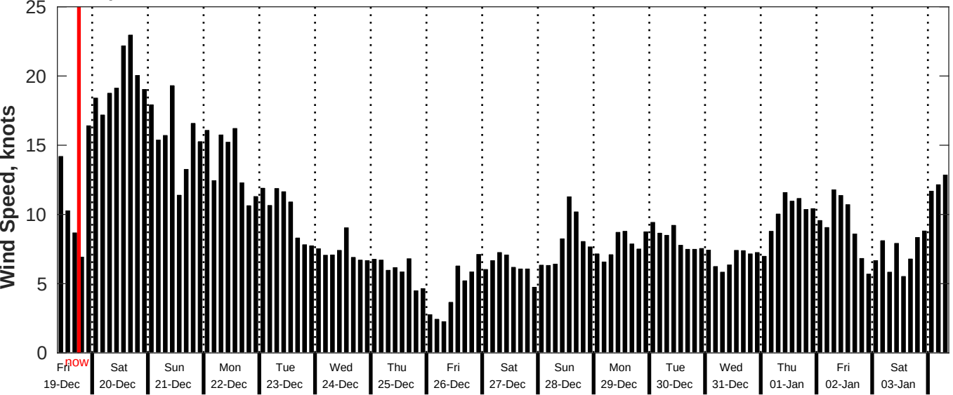
GFS Wind Speed Forecast for NDBC 52212 from 18-Dec-2025 09:00:00 to 03-Jan-2026 09:00:00
