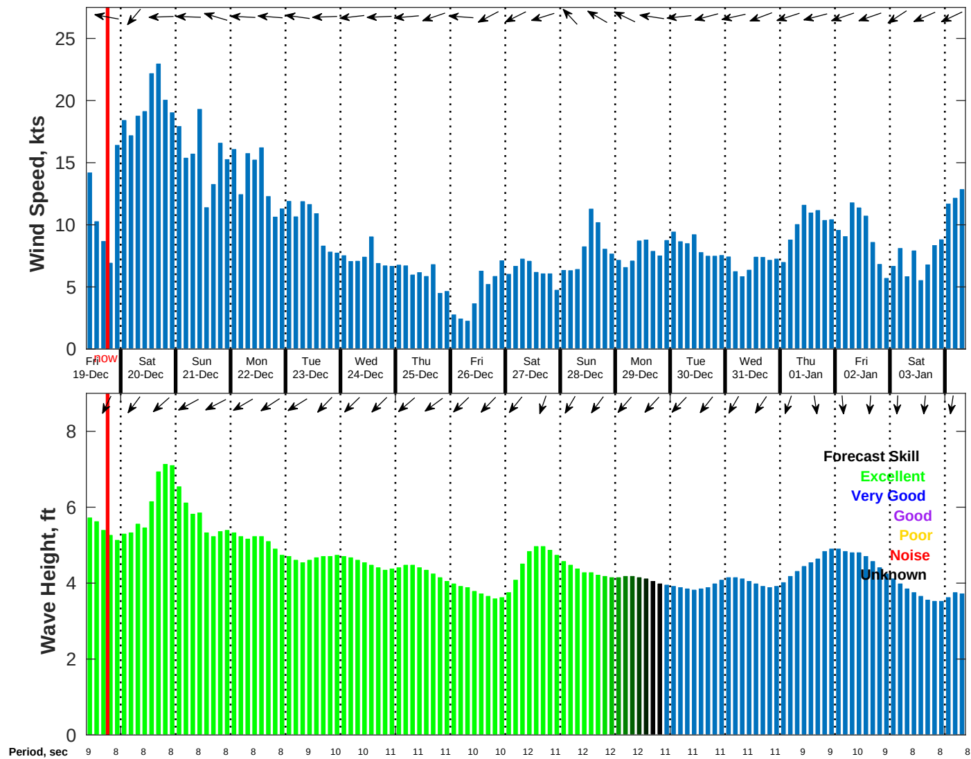
Wind & Wave Forecast for NDBC 52212 from 18-Dec-2025 09:00:00 to 03-Jan-2026 09:00:00
