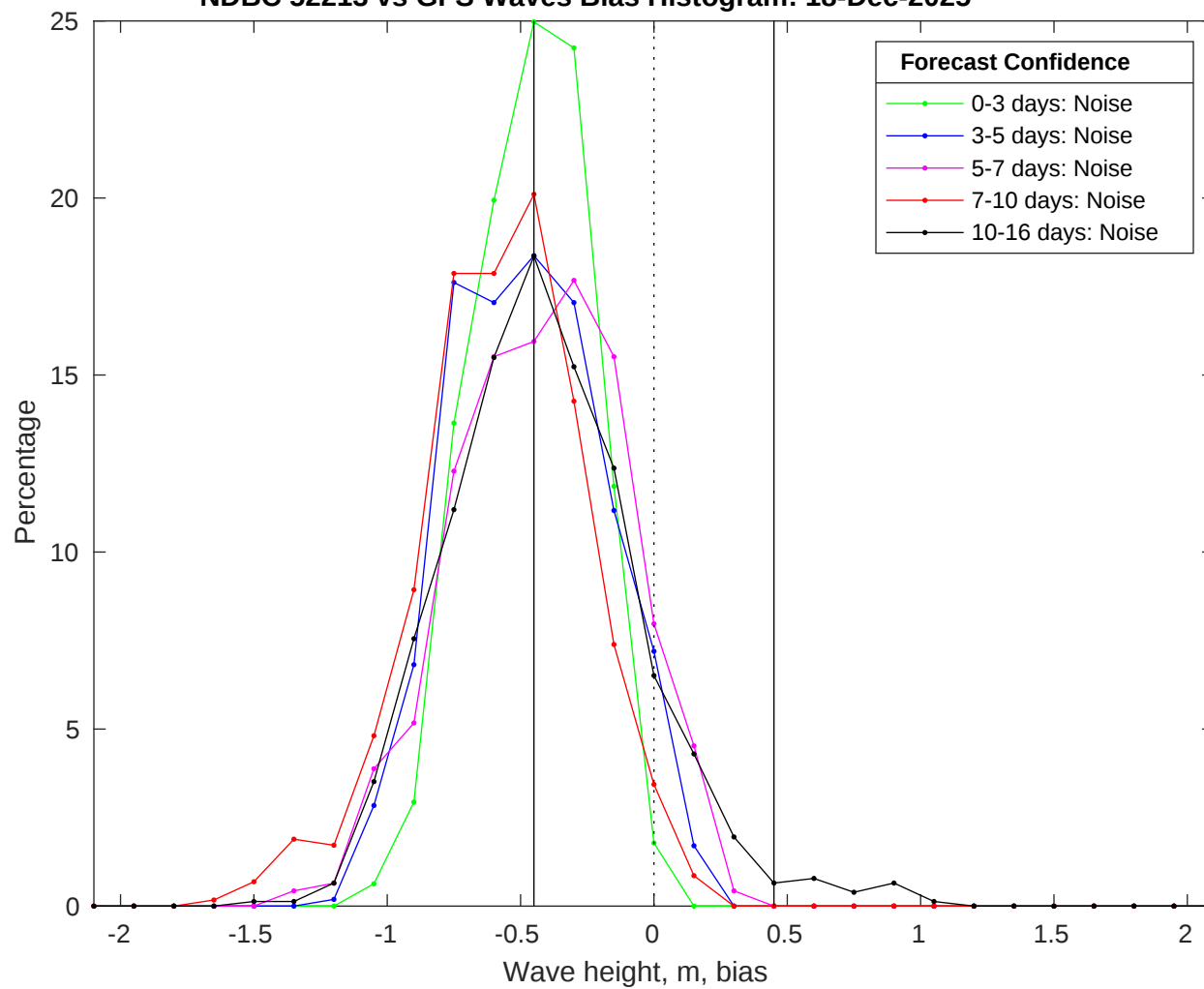
NDBC 52213 vs GFS Waves Bias Histogram: 18-Dec-2025
