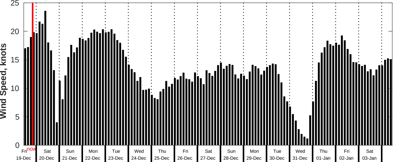
GFS Wind Speed Forecast for NDBC 52213 from 18-Dec-2025 11:00:00 to 03-Jan-2026 11:00:00
