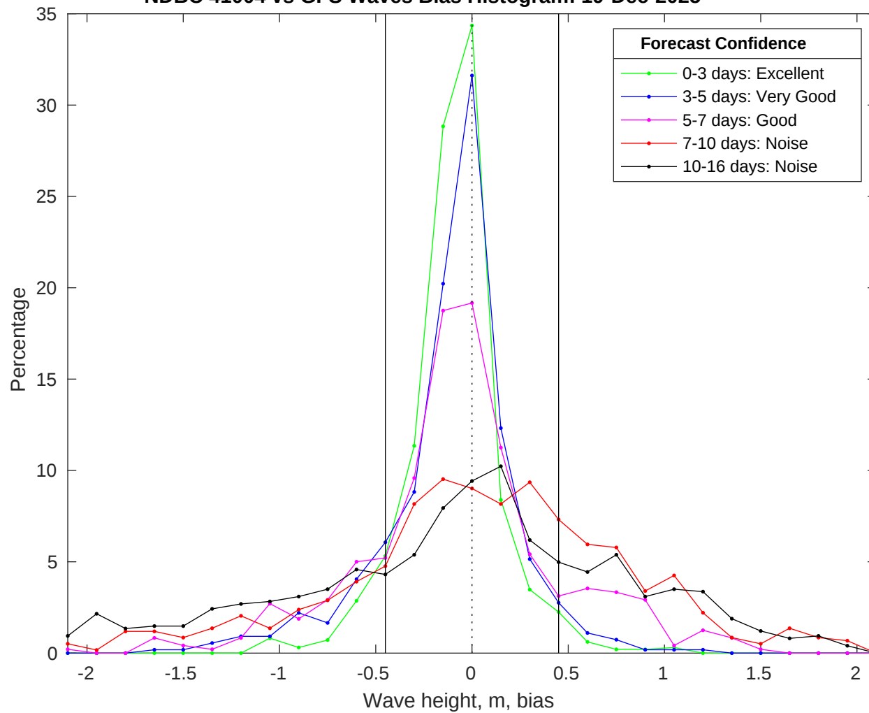
NDBC 41004 vs GFS Waves Bias Histogram: 19-Dec-2025
