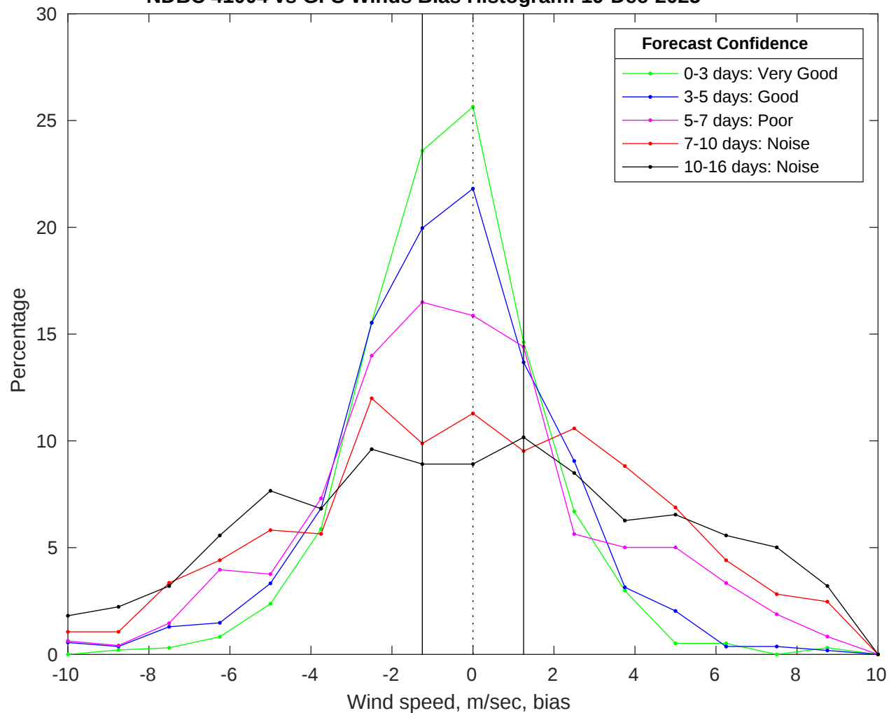
NDBC 41004 vs GFS Winds Bias Histogram: 19-Dec-2025
