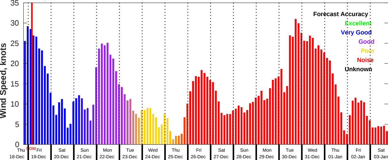
GFS Wind Speed Forecast for NDBC 41004 from 18-Dec-2025 19:00:00 to 03-Jan-2026 19:00:00
