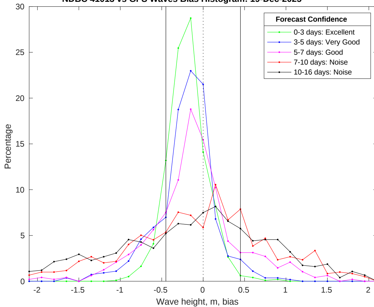
NDBC 41013 vs GFS Waves Bias Histogram: 19-Dec-2025
