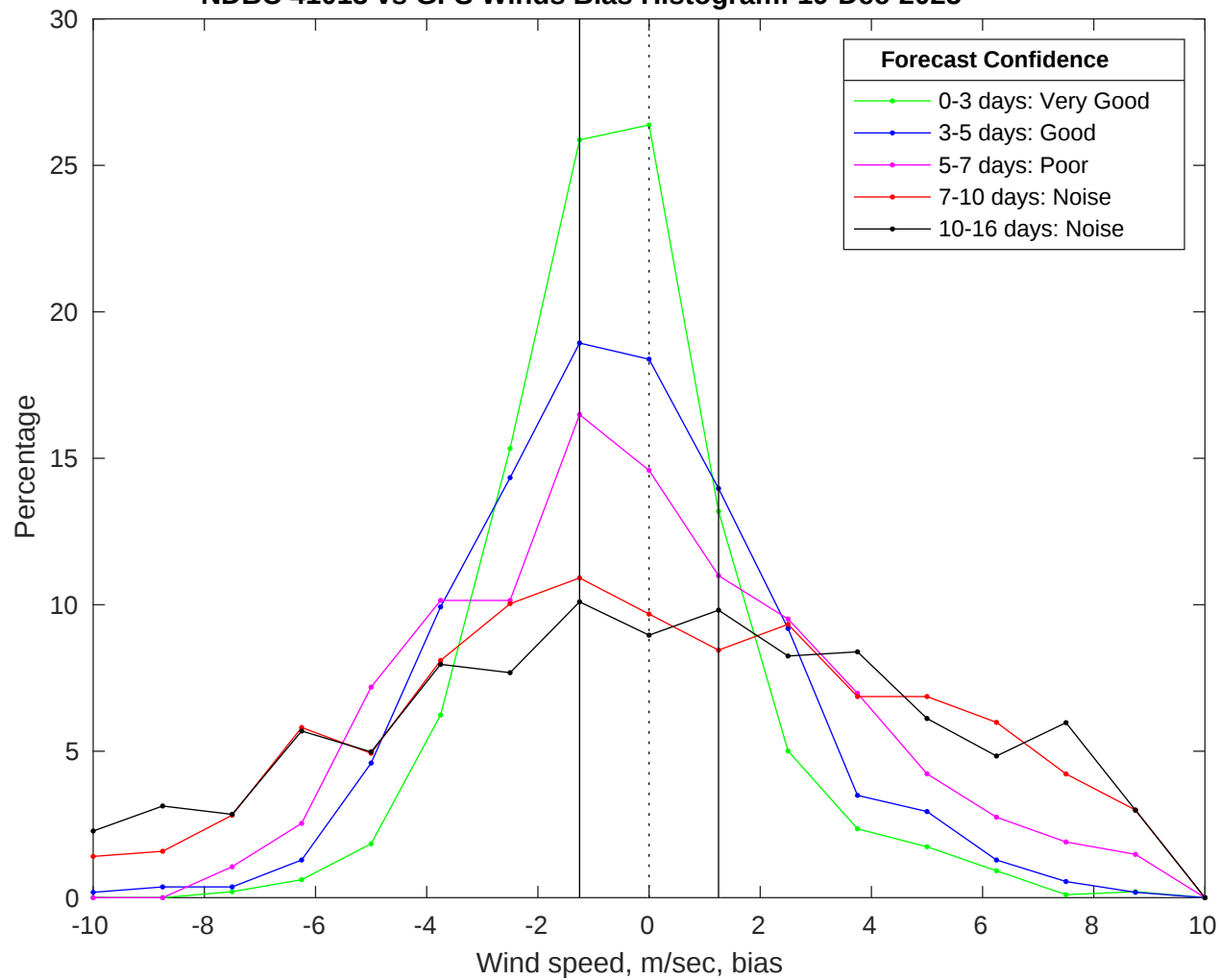
NDBC 41013 vs GFS Winds Bias Histogram: 19-Dec-2025
